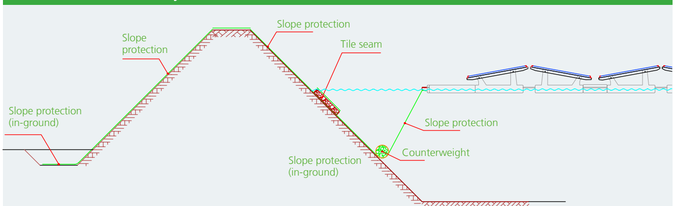
Cross Section Sun on Water System
